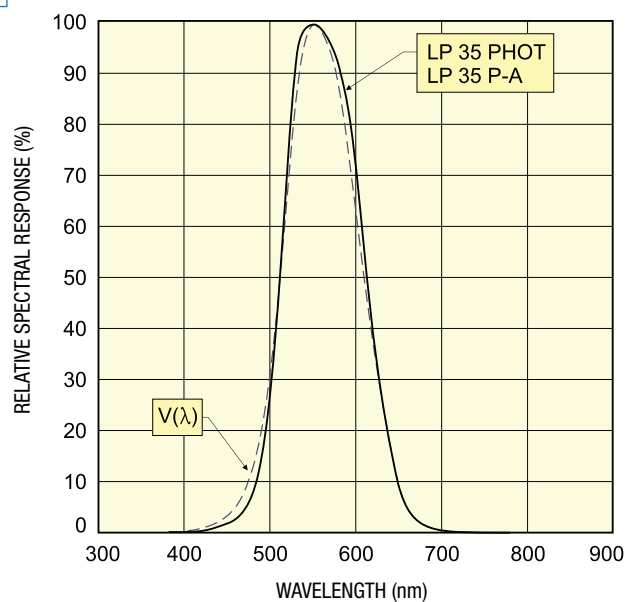
Graph 1 Relative spectral response of the illuminance sensor
