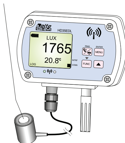
Illuminance and UVA sensor
