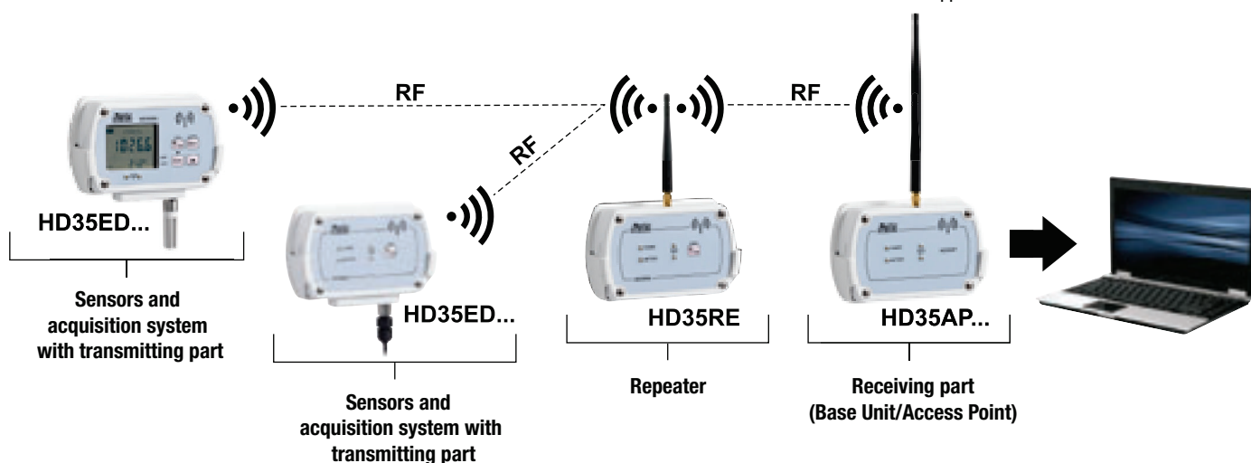
Wireless data recording system with repeater
